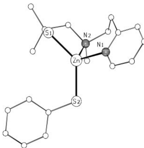
Figure 4. Molecular structure of L 3 ·Zn–SC 6 H 5 ( 3d ). Relevant bond lengths [Å] and angles [°]: Zn–N1 2.076(7), Zn–N2 2.149(9), Zn–S1 2.273(3), Zn–S2 2.277(3); N1–Zn–N2 96.9(3), N1–Zn–S1 113.1(2), N1–Zn–S2 102.3(2), N2–Zn–S1 90.8(2), N2–Zn–S2 116.0(2), S1–Zn–S2 132.4(1).
