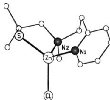
Figure 3. Structure of L 3 ·Zn–Cl. Relevant bond lengths [Å] and angles [°]: Zn–Cl 2.2354(5), Zn–S 2.2532(5), Zn–N1 2.057(1), Zn–N2 2.108(1); N1–Zn–N2 98.96(5), S–Zn–N2 92.72(4), Cl–Zn–N2 116.38(4), S–Zn–N1 120.09(4), Cl–Zn–N1 101.66(4), Cl–Zn–S 124.55(2).
