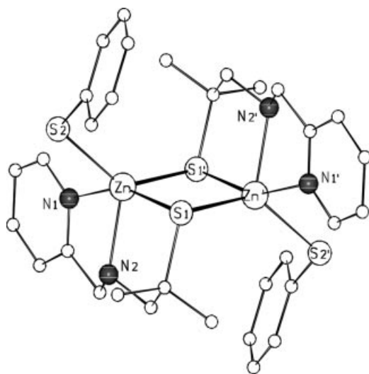
Figure 1. Structure of 1 in the solid state. Relevant bond lengths [ \text{\AA} ]: Zn–S1 2.514(2), Zn–S1' 2.370(2), Zn–S2 2.321(2), Zn–N1 2.305(4), Zn–N2 2.134(4).
