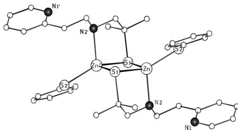
Figure 2. Structure of 2a in the solid state. Relevant bond lengths [Å] and angles [°]: Zn–S1 2.375(4), Zn–S1' 2.377(4), Zn–S2 2.254(3), Zn–N2 2.101(5); S1–Zn–S1' 99.3(1), Zn–S1–Zn' 80.7(1), S1–Zn–N2 90.1(1), S1–Zn–S2 130.0(1).
